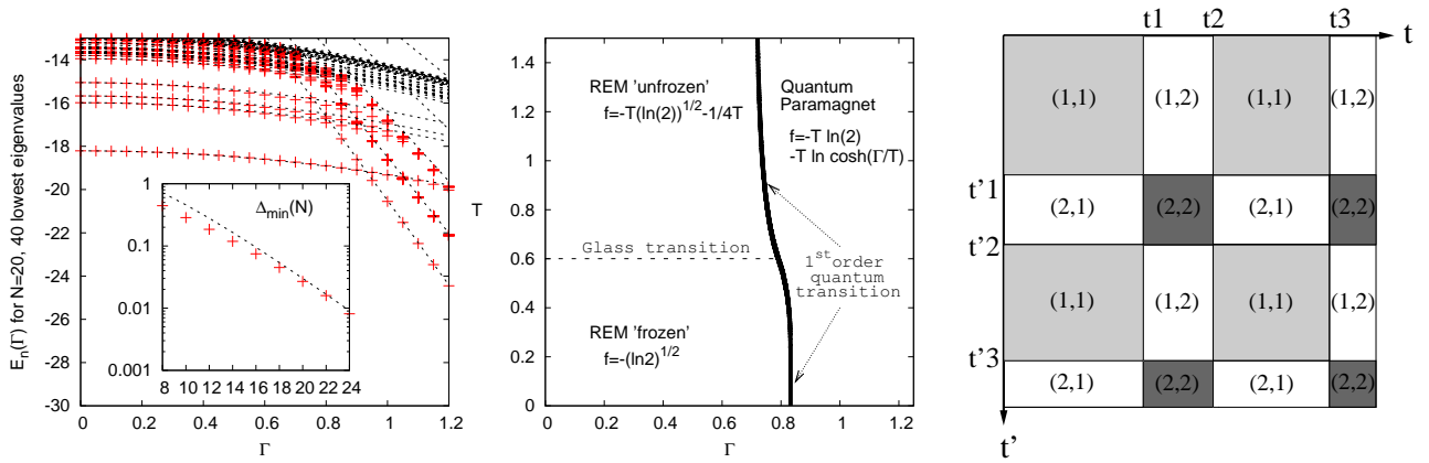
FIG. 1: Left: Evolution of lowest energy Levels for a single realization of the QREM with N = 20 spins (dots) compared with analytical predictions (lines). Inset: evolution of the ensemble averaged minimal gap at the transition. Center: Phase diagram of the QREM in temperature T and transverse quantum field \Gamma . At T = 0 the quantum transition arises at \Gamma_c = \sqrt{\ln 2} while the classical glass transition for \Gamma = 0 is at T_c = 1/2\sqrt{\ln 2} . Right: A multi-instanton configuration for the two-times overlap q_{t,t'} and the two-time Lagrange multipliers \tilde{q}_{t,t'} . Far from the jump times, the functions q_{t,t'} and \tilde{q}_{t,t'} take the same form as those computed at those times for the glass phase (the regions (1,1)), for the quantum paramagnet (in the regions (2,2)), and are zero in the mixed regions (1,2)-(2,1). In the large p limit the problem can be solved completely using the so-called ‘static approximation’ [5, 14] within the (1,1) regions, and, in addition, the fact that \tilde{q}_{t,t'}^d and \tilde{q}_{t,t'} become either infinity or zero, with sharp interfaces.
