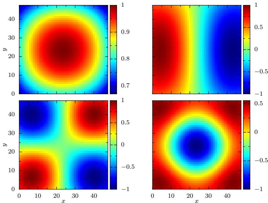
Figure 8. Amplitudes of modes found in a square observation window 48 \times 48 pixels, using scalar elasticity. Top left to bottom right decreasing eigenvalues of the integral operator. Note that first mode is not constant within the observation volume despite it being the most uniform mode. The second mode displays a noticeable non-sinusoidal form.
