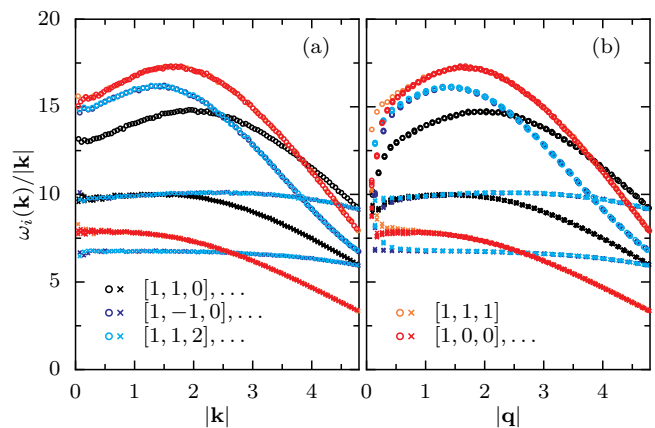
Figure 5. As Fig. 2 but using a Hann window in (b). The windowing artefacts are largely eliminated, but the three longest wavelength modes are modified due to mode mixing, compare Appendix A. Skew window adapted to simulation box.
