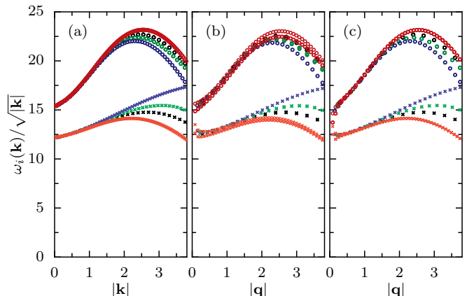
Figure 7. Projected dispersion curves from the simulation in Fig. 2. The projected system is two-dimensional and isotropic. (a) full system, (b) truncation window, (c) window with Hann weighting functions, see eq. (26).
