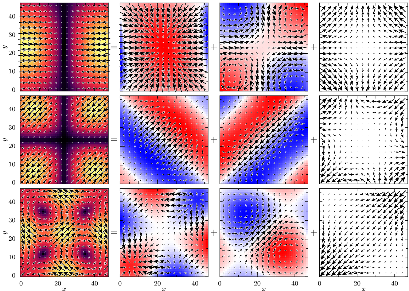
Figure 9. Three eigenmodes of the truncated system: Left panels show the displacement field, colours indicate absolute value (black=small, yellow=large). The three columns on the right show the Helmholtz–Hodge decomposition into longitudinal, transverse and harmonic parts. The blue/red colour shows the divergence (second column) and the rotation (third column) of the displacement field (red=negative, blue=positive). \lambda = \mu .
