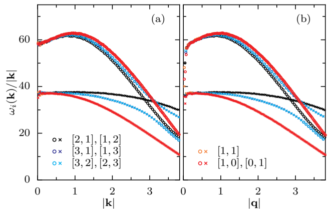
Figure 4. As Fig. 1 but using a Hann window in (b). The windowing artefacts are largely eliminated, but the three longest wavelength modes are modified due to mode mixing, See Appendix A. Skew window adapted to simulation box.
