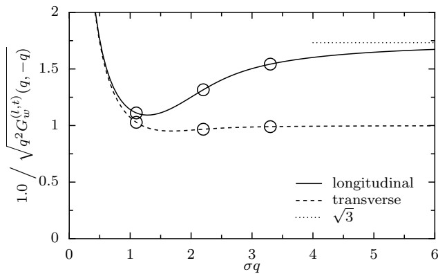
Figure 6. Effective \omega/q for a three dimensional system with \lambda/\mu = 1 , \nu = 0 , analysed using a Gaussian window of variance \sigma^2 . For large values of \sigma q the ratio of the two curves converges to the expected value \sqrt{3} . However mixing of the modes leads to a strong drop in the estimate of the longitudinal stiffness for \sigma q \approx 1 . Symbols correspond to the first three modes using a corresponding Hann window.
