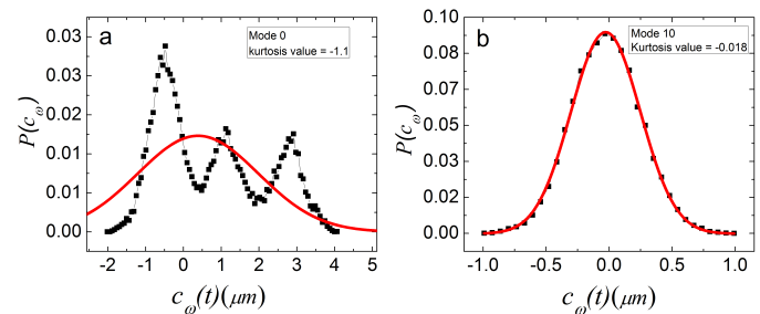
FIG. 1: (color online) Distribution of instantaneous projection coefficient c_\omega(t) for a. the lowest frequency mode, mode 0; and b. the 10th lowest frequency mode. Red lines are Gaussian fits to the distributions.
