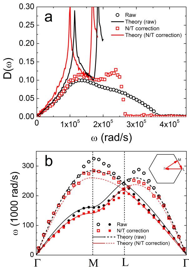
FIG. 3: (color online) a. Phonon density of states of two dimensional colloidal crystals. DOS obtained from experimental data (black circles), and DOS after N/T extrapolation (red squares). Numerically generated DOS for the harmonic triangular lattice (with matched sound speeds) is plotted as a guide of eye (solid lines). b. Dispersion curves for longitudinal (open symbols) and transverse modes (filled symbols) along high-symmetry directions, including uncorrected experimental data (black circles), and data after N/T extrapolation (red squares). Theoretical expectations are plotted in dashed (longitudinal) and solid (transverse) lines with matched colors. Inset: high symmetry directions in reciprocal space.
