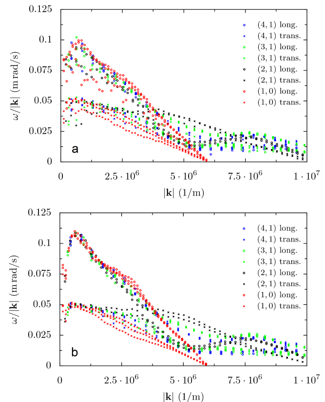
FIG. 5: (color online) Correction for limited field of view. a. Dispersion curves along different directions derived from uncorrected data. Circles represent longitudinal modes and crosses represent transverse modes. Directions are indexed using the basis vectors of the reciprocal lattice. b. Dispersion curves along different directions after the Hann window function correction.
