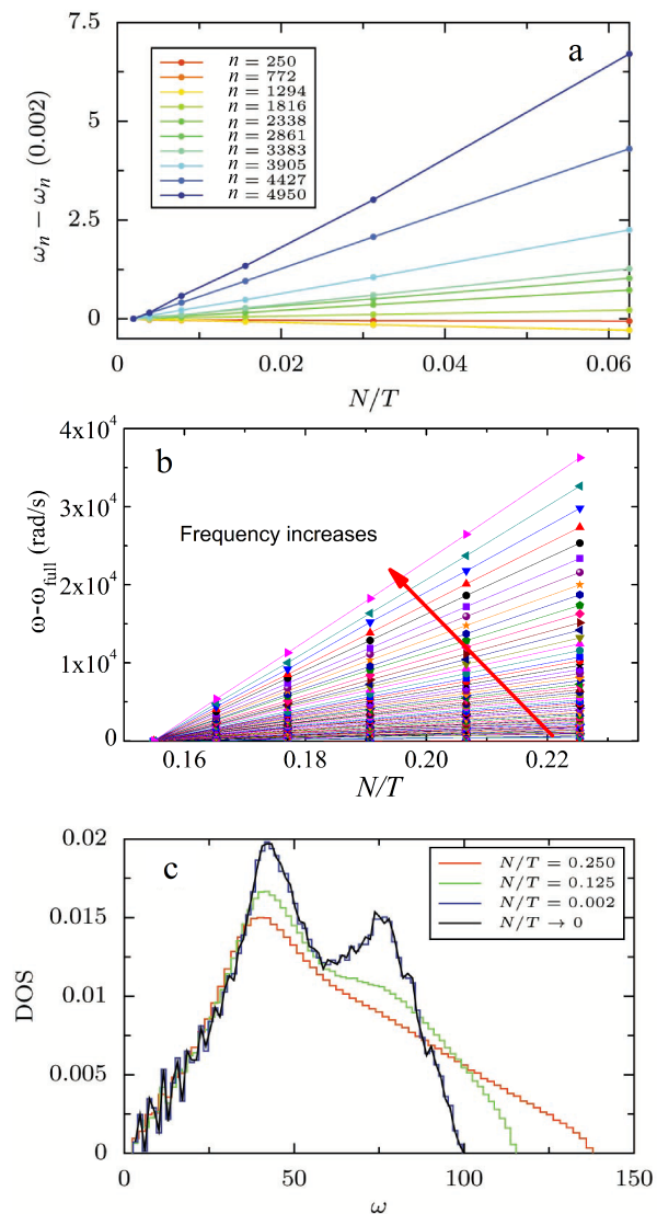
FIG. 4: (color online) Correction for a finite number of observation frames. a. Linear dependence of eigenfrequencies on N/T from simulation. n is the mode index which increases from low to high frequencies. For better visualization, a constant, the corresponding mode frequency for R = 0.002 , has been subtracted for each curve. b. Linear convergence of eigenfrequencies from experimental data with N/T . The vertical axis plots the frequencies minus the frequency from the full length of the video, \omega_{full} . c. Density of states for different ratios of N/T from simulation.
